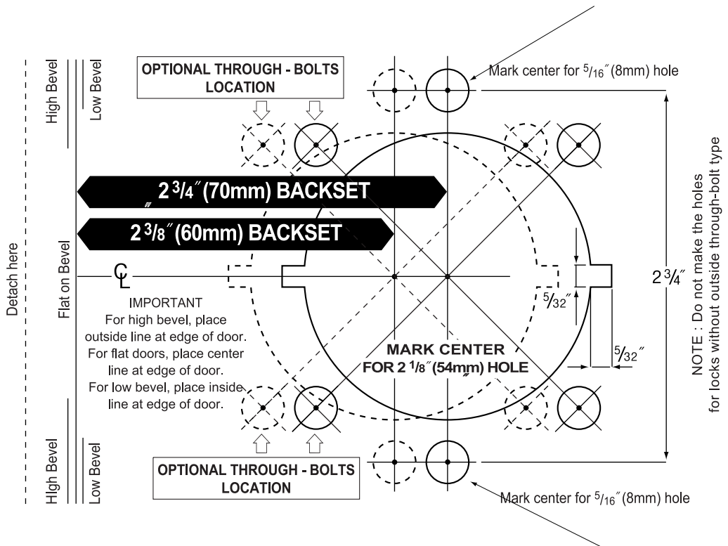
INSTALLATION TEMPLATE
