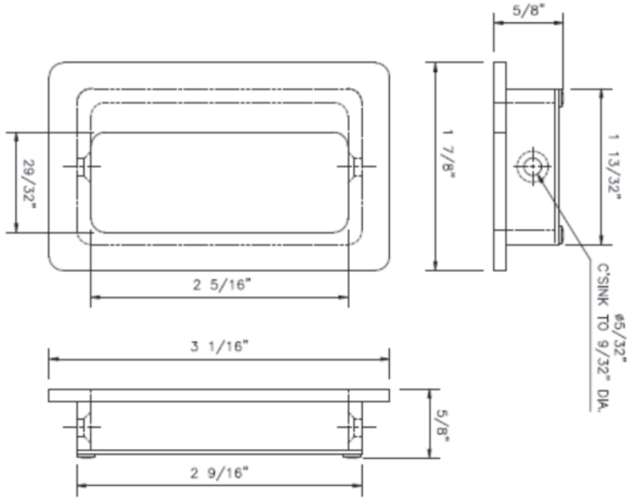
960 - FLUSH PULL
