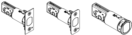
Square corner 1/4" Radius Drive-in
