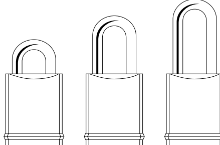
3/4" 1 1/2" 2" 20 Series 5/16" Shackle diameter
